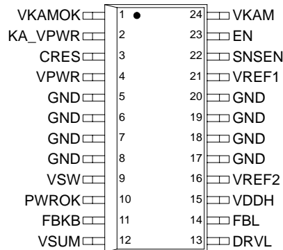
Figure 3. 33997 Pin Connections
