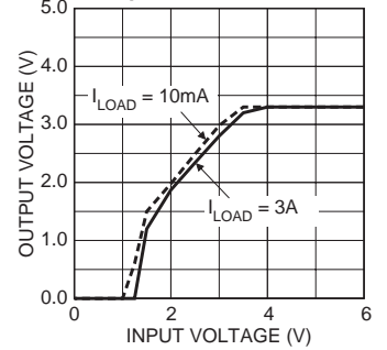
MIC29310-3.3 Dropout Characteristics
