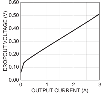
MIC2931x Dropout Voltage vs. Output Current
