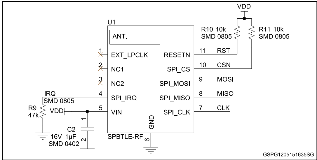
Figure 3: Nucleo connections
