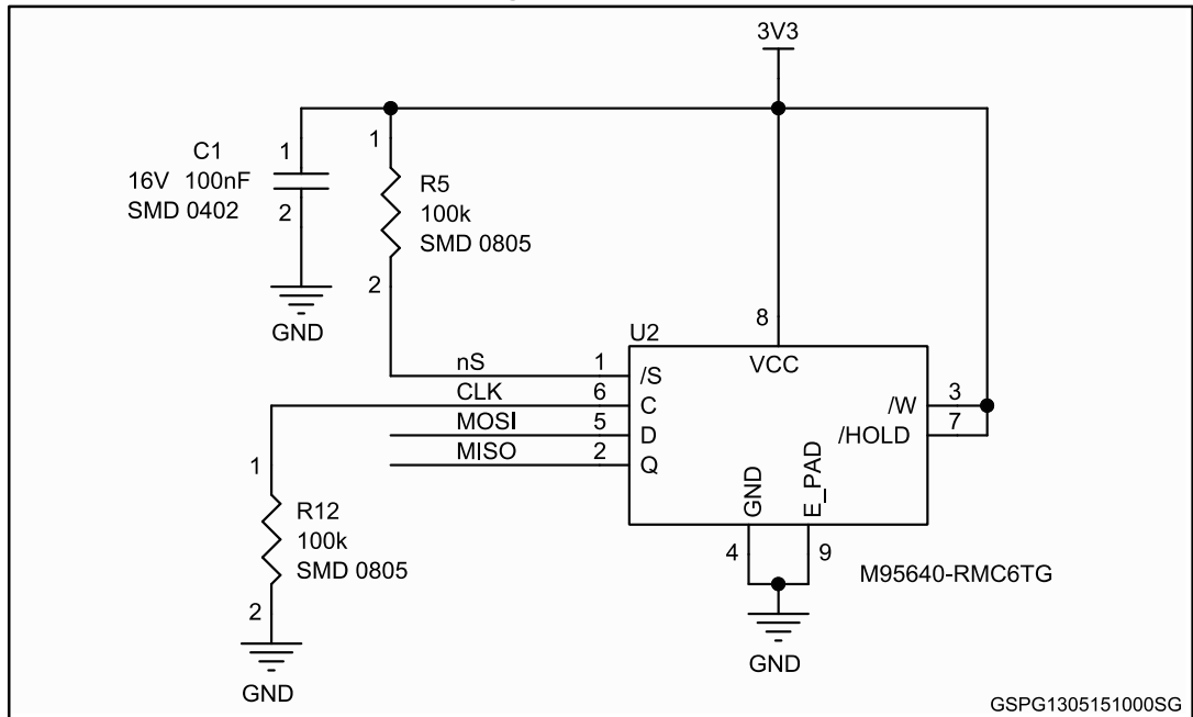
Figure 4: EEPROM
