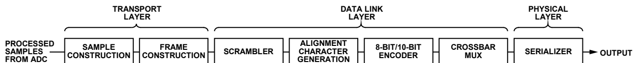
Figure 87. Data Flow
