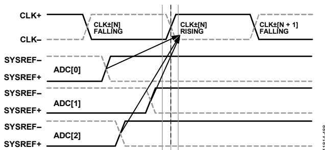
Figure 103. Changing the Latching Edge to Rising for All Three ADCs, \text{SYSREF}_{\pm} Can Now be Aligned to \text{CLK}_{\pm}[N]
