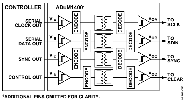
Figure 58. Isolated Interface
