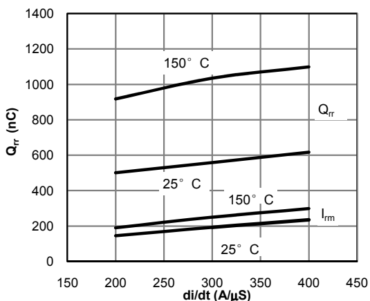
Fig 23: Diode Reverse Recovery Charge and Peak Current vs. di/dt ( V_{GE}=15V, V_{CE}=400V, I_F=15A )
