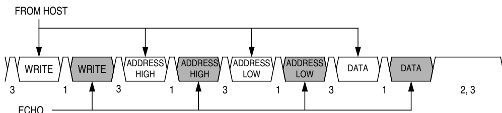
Figure 8-5. Read Transaction
