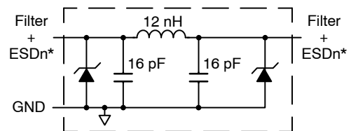
1 of 4, 6 or 8 EMI/RFI Filter Channels with Integrated ESD Protection
