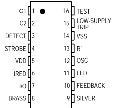
Figure 1. Pin Connections
