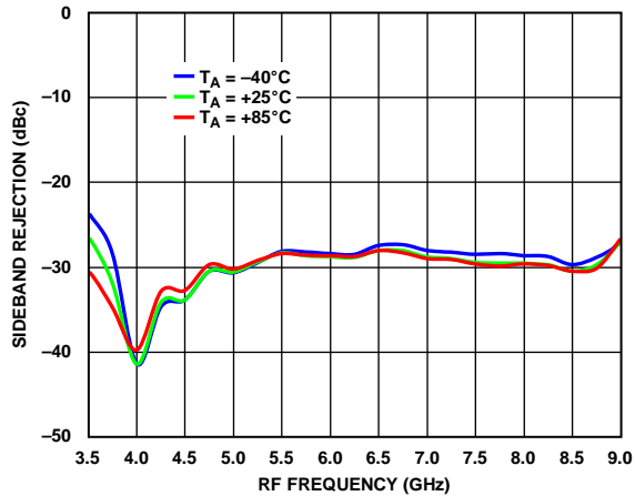
Figure 53. Sideband Rejection vs. RF Frequency at Various Temperatures, LO = 15 \text{ dBm}
