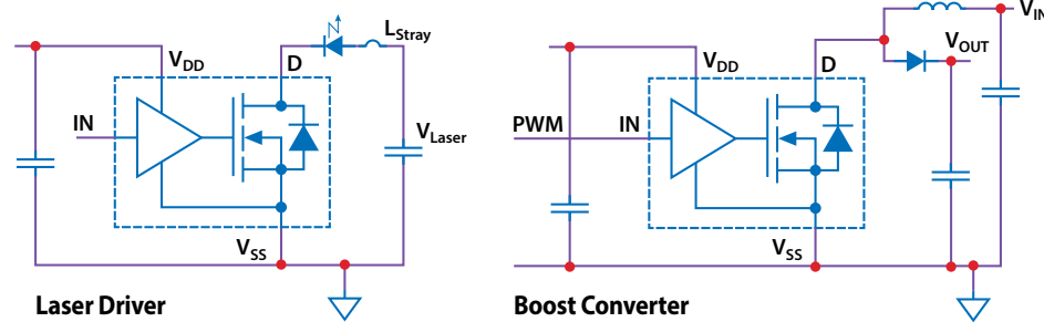
Figure 1: Typical Connection Diagrams
