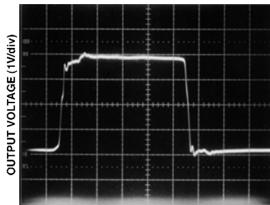
V_S = \pm 5V R_F = R_G = 1k\Omega R_L = 150\Omega A_V = +2 TIME (20 ns/div)
