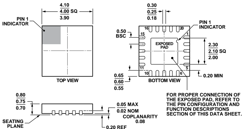
Figure 12. 20-Lead Lead Frame Chip Scale Package [LFCSF_WQ] 4 mm × 4 mm Body, Very Very Thin Quad (CP-20-6)
