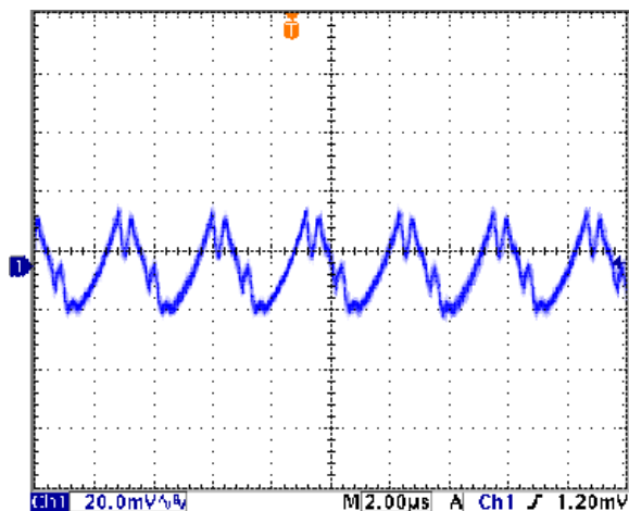
Output Ripple and Noise (Vin=5V, Vout=3.3V, Iout=16A, Cload=0, ScopeBW=100MHz)
