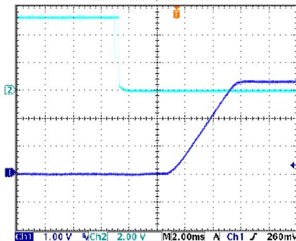
On/Off Enable Startup Delay (Vin=5V, Vout=3.3V, Iout=16A, Cload=0) Trace 2=Enable In, Trace 1=Vout
