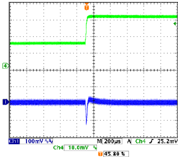
Step Load Transient Response ( V_{in}=5V, V_{out}=2.5V, \text{Load}=0, I_{out}=8A \text{ to } 16A ) Trace 1=Vout, 100 mV/div. Trace 4=Iout, 5A/div.
