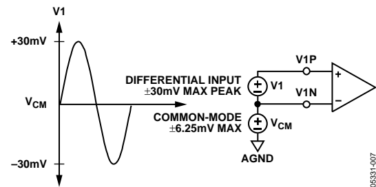
Figure 18. Maximum Signal Levels, Channel V1
