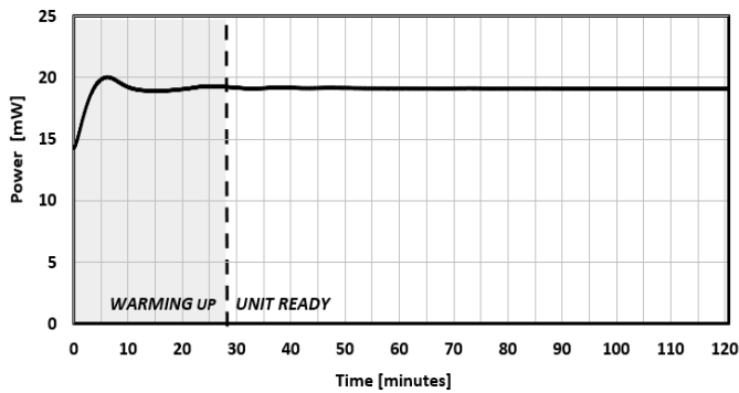
FIG. 9: WARM-UP TIME
