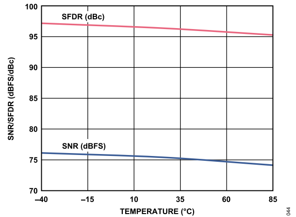
Figure 40. SNR/SFDR vs. Temperature, f_{IN} = 10.3 \text{ MHz} , f_{SAMPLE} = 125 \text{ MSPS}
