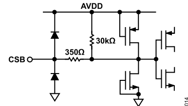
Figure 53. Equivalent CSB Input Circuit
