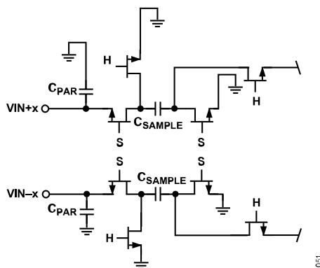
Figure 55. Switched-Capacitor Input Circuit
