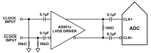
Figure 66. Differential LVDS Sample Clock (Up to 1 GHz)
