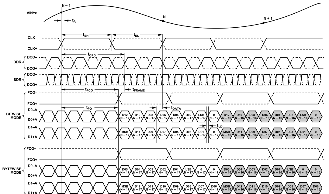
Figure 2. 16-Bit DDR/SDR, Two-Lane, 1x Frame Mode (Default)
