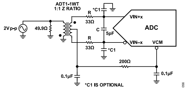
Figure 59. Differential Transformer-Coupled Configuration for Baseband Applications
