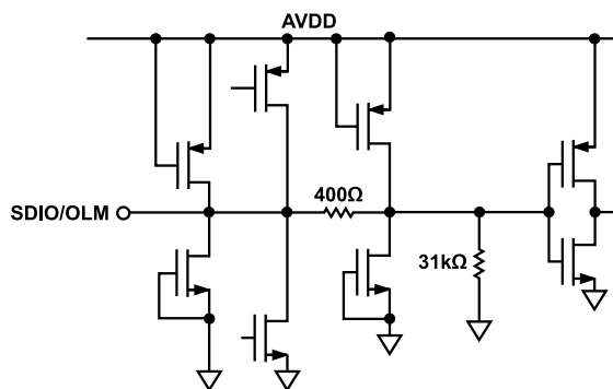
Figure 49. Equivalent SDIO/OLM Input Circuit
