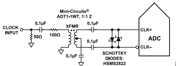
Figure 62. Transformer-Coupled Differential Clock (Up to 200 MHz)
