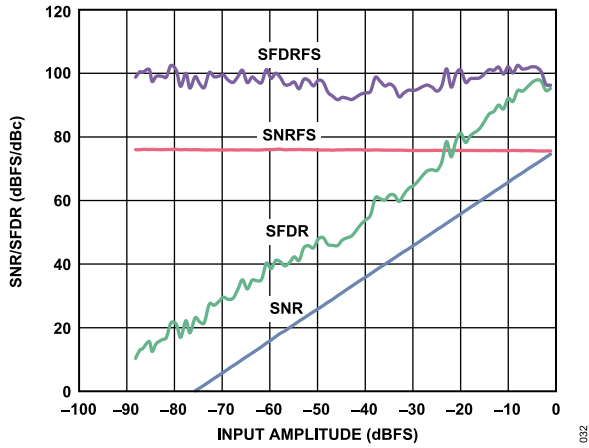
Figure 36. SNR/SFDR vs. Analog Input Level, f_{IN} = 9.7 \text{ MHz} , f_{SAMPLE} = 125 \text{ MSPS}
