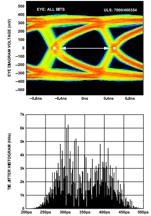
Figure 72. Data Eye for LVDS Outputs in ANSI-644 Mode with Trace Lengths Less than 24 Inches on Standard FR-4 Material, External 100 Ω Far-End Termination Only
