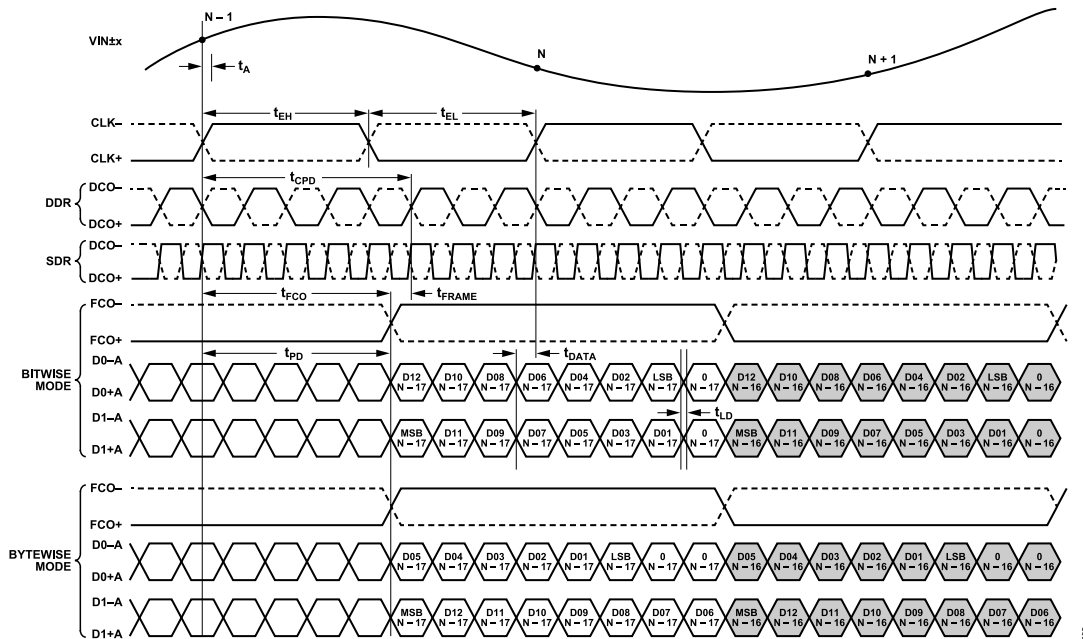
Figure 4. 16-Bit DDR/SDR, Two-Lane, 2x Frame Mode
