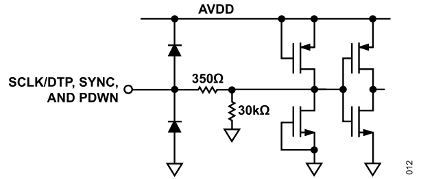
Figure 51. Equivalent SCLK/DTP, SYNC, and PDWN Input Circuit
