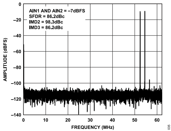
Figure 37. Two-Tone 16k FFT with f_{IN1} = 70.5 \text{ MHz} and f_{IN2} = 72.5 \text{ MHz} , f_{SAMPLE} = 125 \text{ MSPS}
