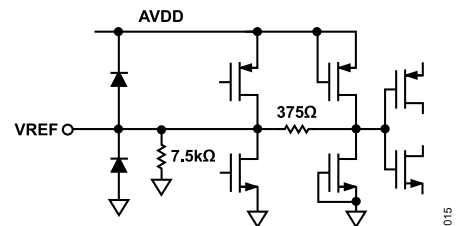
Figure 54. Equivalent VREF Circuit
