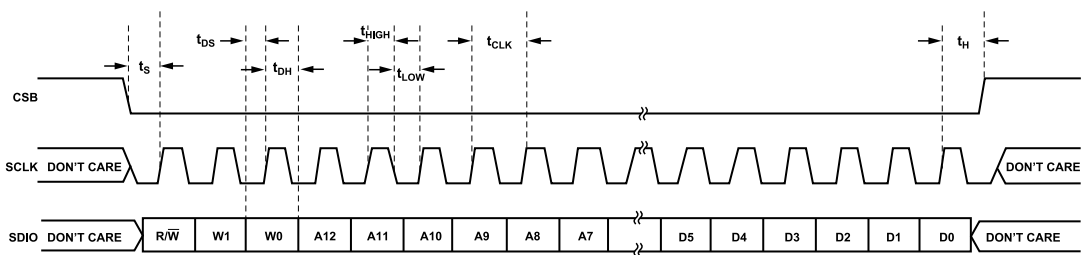
Figure 74. Serial Port Interface Timing Diagram
