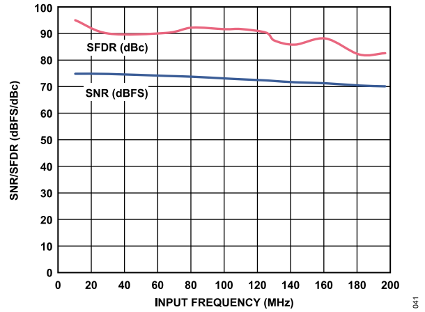
Figure 39. SNR/SFDR vs. f_{IN} , f_{SAMPLE} = 125 \text{ MSPS}
