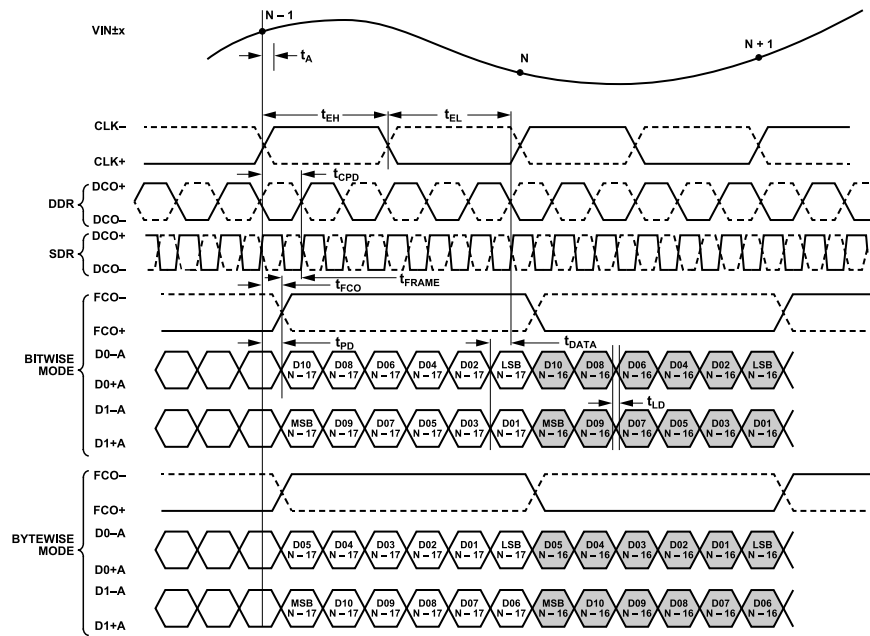
Figure 5. 12-Bit DDR/SDR, Two-Lane, 2x Frame Mode
