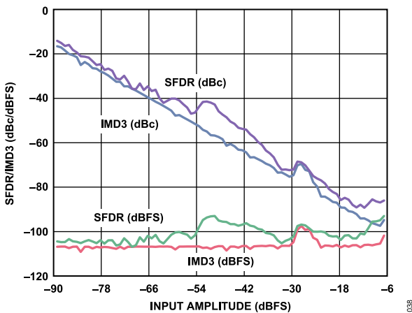
Figure 38. Two-Tone SFDR/IMD3 vs. Input Amplitude (AIN) with f_{IN1} = 70.5 \text{ MHz} and f_{IN2} = 72.5 \text{ MHz} , f_{SAMPLE} = 125 \text{ MSPS}
