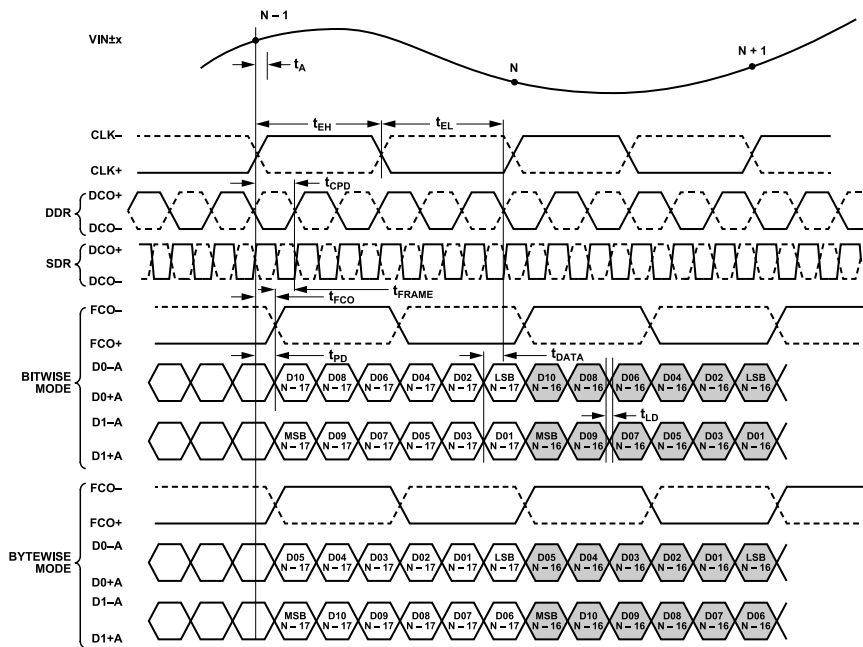
Figure 3. 12-Bit DDR/SDR, Two-Lane, 1x Frame Mode
