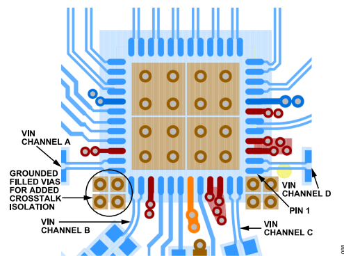
Figure 76. Layout Technique to Maximize Crosstalk Performance
