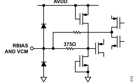
Figure 52. Equivalent RBIAS and VCM Circuit
