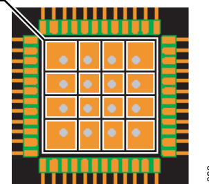
Figure 75. Typical PCB Layout
