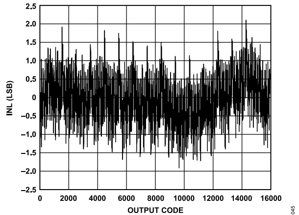
Figure 41. INL, f_{IN} = 9.7 \text{ MHz} , f_{SAMPLE} = 125 \text{ MSPS}
