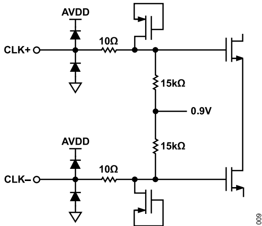
Figure 48. Equivalent Clock Input Circuit
