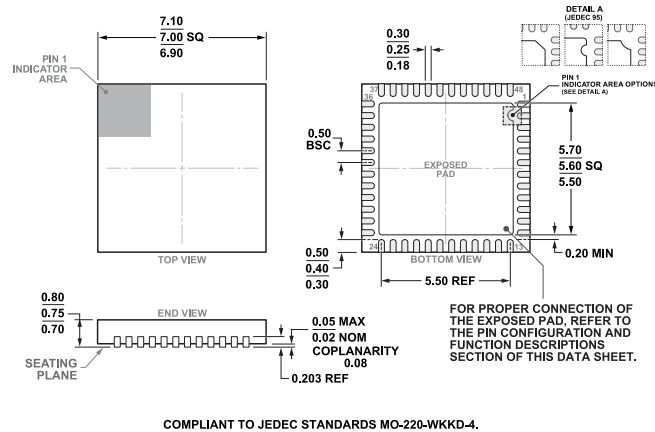
Figure 77. 48-Lead Lead Frame Chip Scale Package [LFCSP] 7 mm x 7 mm Body and 0.75 mm Package Height (CP-48-13) Dimensions shown in millimeters
