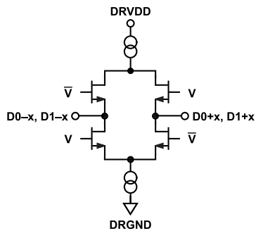
Figure 50. Equivalent Digital Output Circuit
