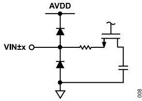
Figure 47. Equivalent Analog Input Circuit
