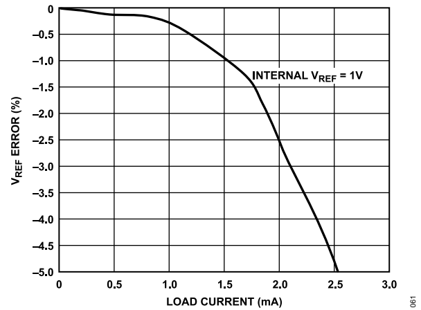
Figure 60. V_{REF} Error vs. Load Current
