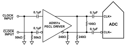
Figure 65. Differential PECL Sample Clock (Up to 1 GHz)
