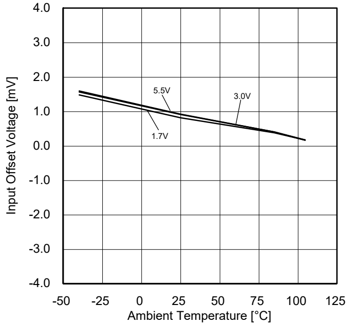
Figure 15. Input Offset Voltage vs Ambient Temperature ( V_{ICM}=V_{DD}-1.2V , E_k=-V_{DD}/2 )
